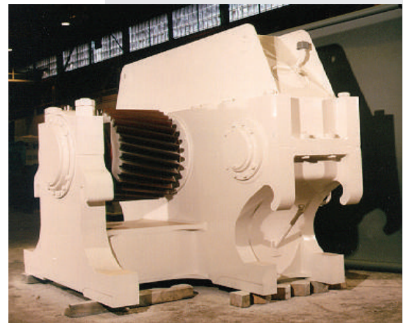
The thick side walls prevent flexing and gear misalignment.
